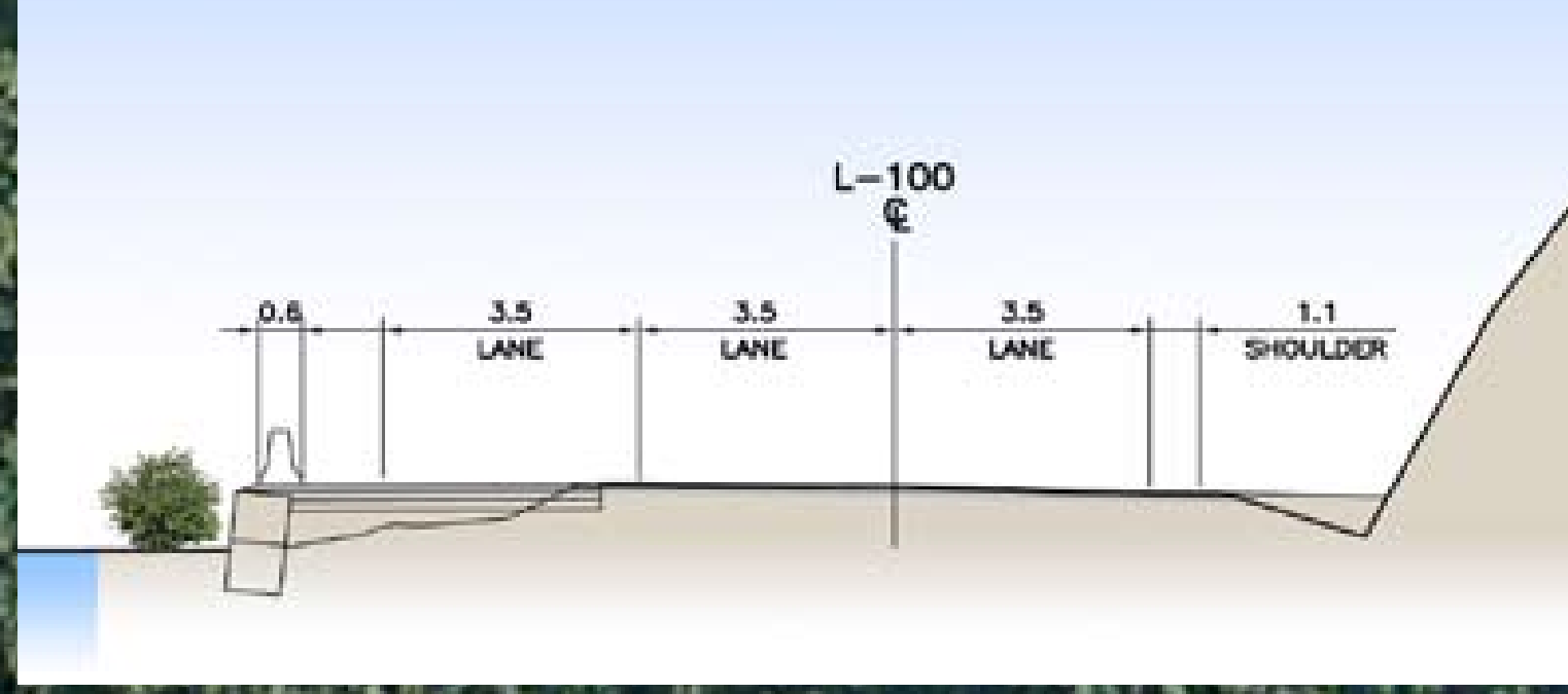
Cross section showing temporary Olympic laning
