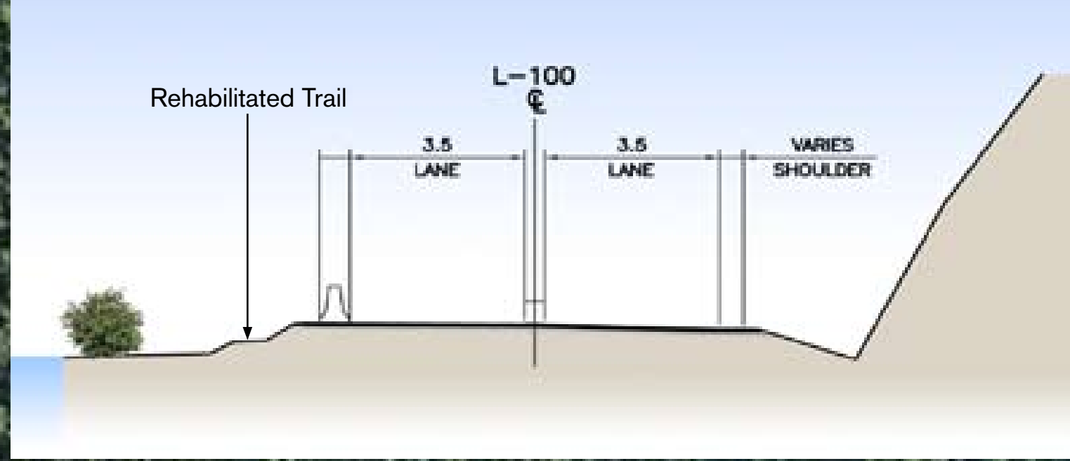
Cross section showing permanent laning in 2010
